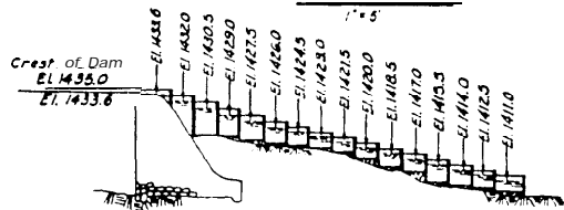
SECTION B-B 1" = 20'
