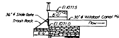
SECTION A-A 1/2" = 1'-0"
