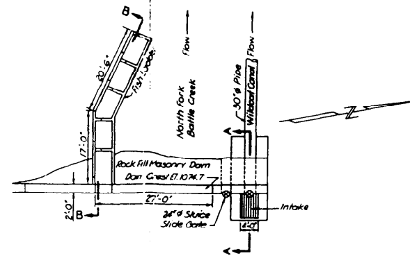
PLAN OF DIVERSION DAM 1'-10'
