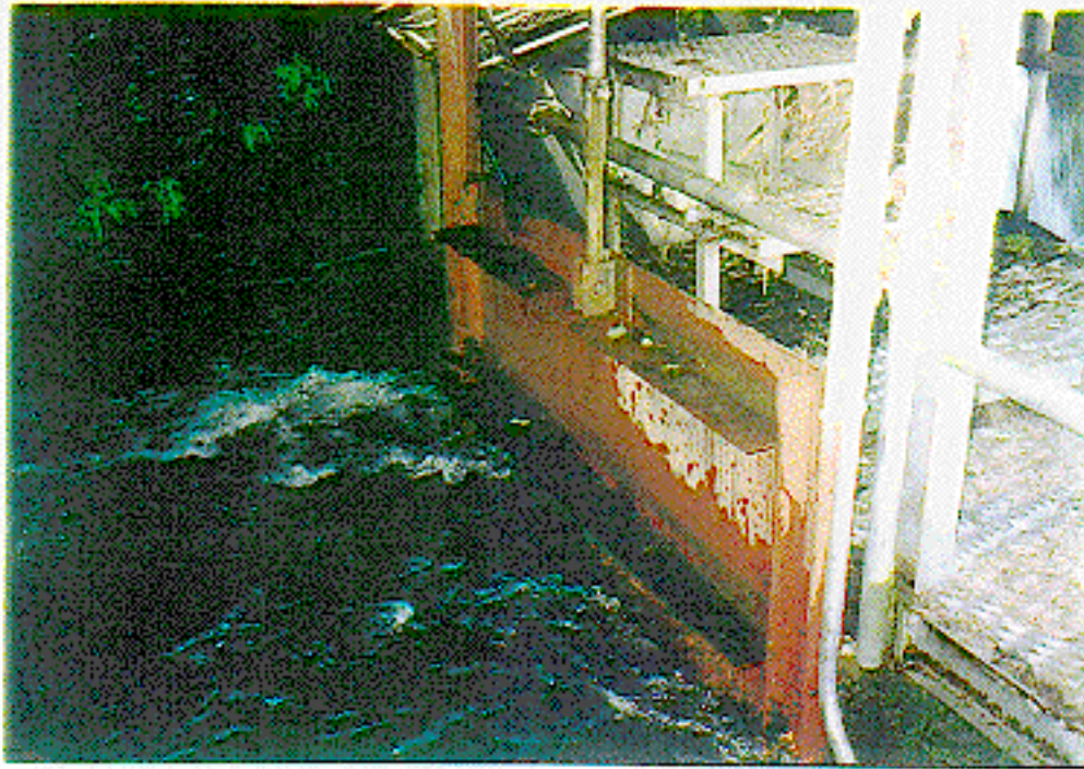
Photograph 3. - Eagle Canyon Dam. 3.5- by 6-foot canal slide gate.
