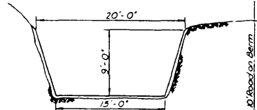
LINED CANAL SECTION 1'-6" Length 15328'
