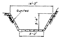
LINED CANAL SECTION Length 12,075' 1" = 5"
