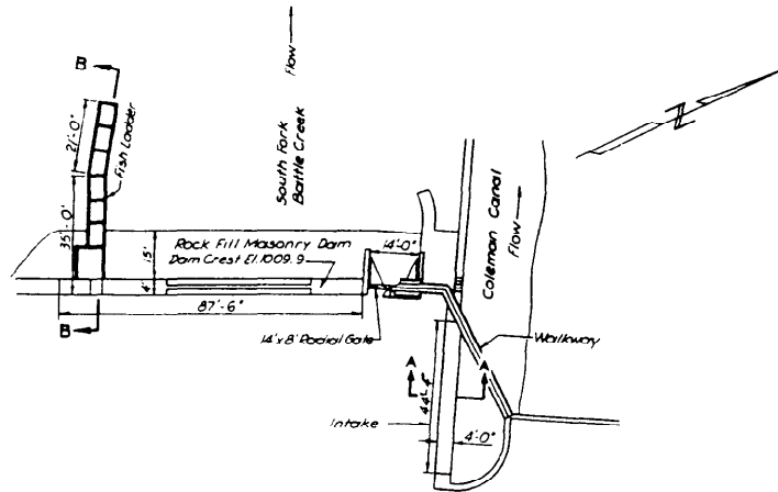
PLAN OF DIVERSION DAM 1'-20'
