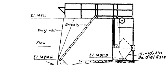
SECTION A-A 1" = 5"
