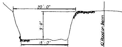
UNLINED CANAL SECTION 1'-6" Length 30912'
