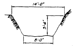
UNLINED CANAL SECTION Length 6466' 1" = 5"
