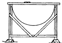
FLUME SECTION 1'-6" #26" d Metal Flume Length 83'
