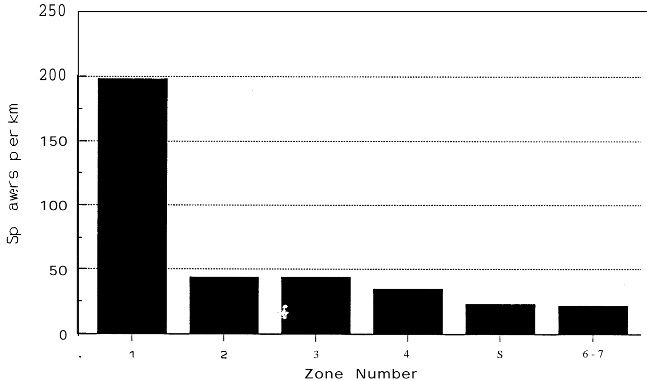
FIGURE 7. Adult chinook salmon spawning density, in spawners per river km, observed in the 1990-91 mainstem Trinity River spawner survey.
